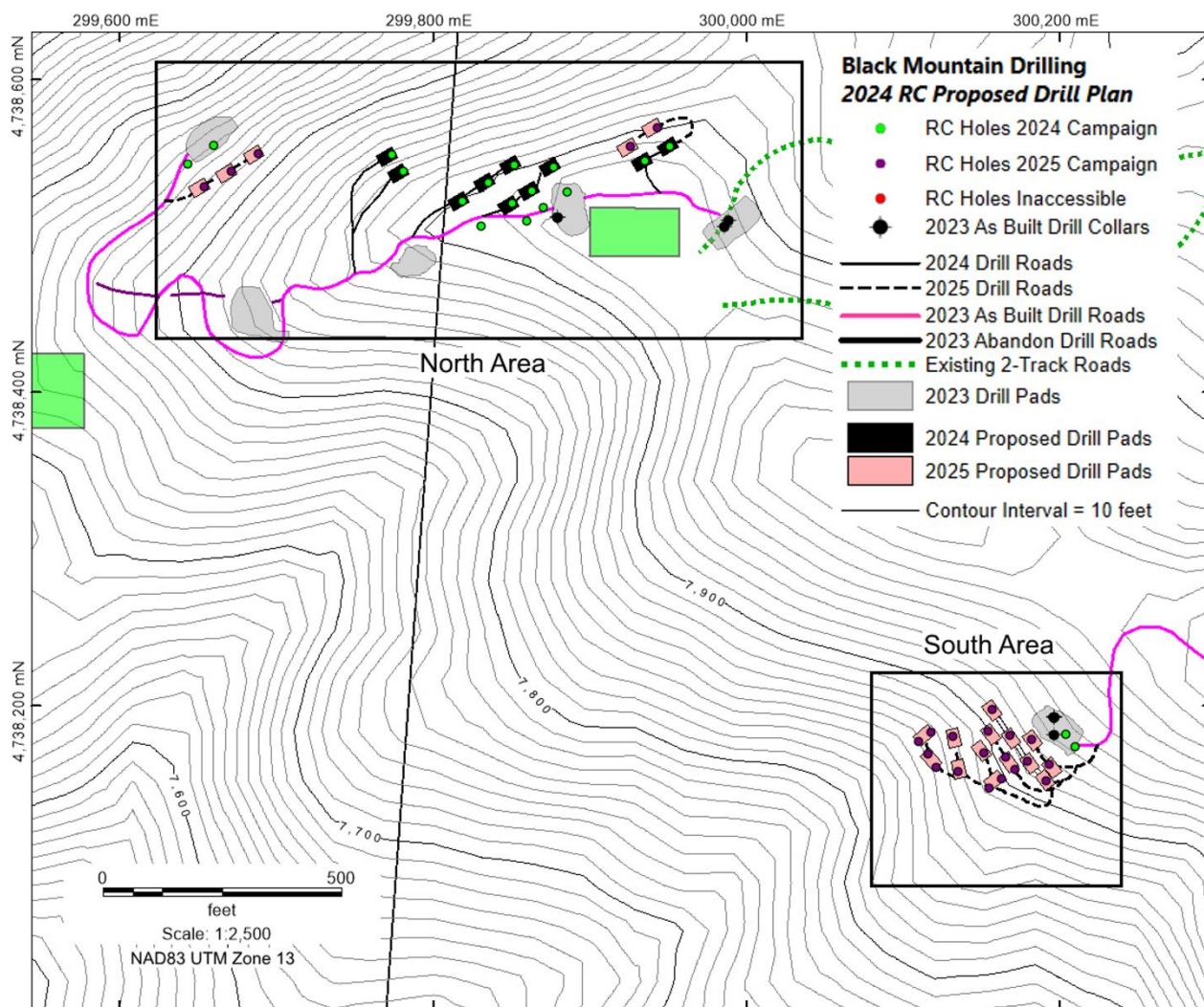
Figure 1: Phase 2 Drill Program Layout
